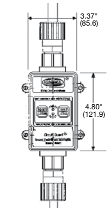
Dimensional Drawing
