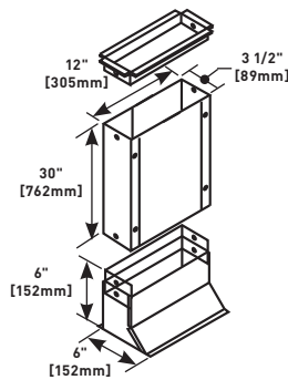
CBR-LT (Access to Two Communication Compartments)
