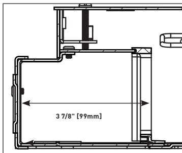
EFB6-0G Depth Behind Plates
