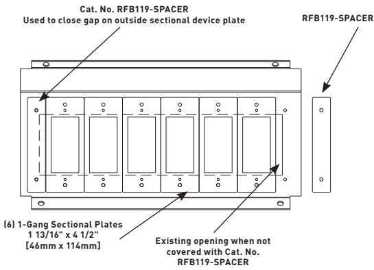
Multi-Gang Mounting Brackets Used with Sectional Device Plates
