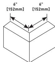
AL3018 External Elbow with Coupling
