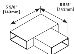
AL3015 Flat Tee
