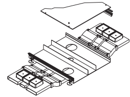
Trenchduct Crossunder Feed into Walkerduct Pro Series
