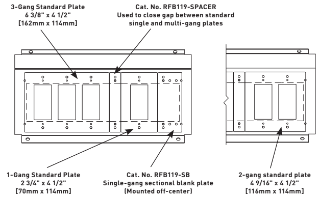
Multi-Gang Mounting Brackets Used with Standard Device Plates
