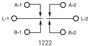
Double Pole Double Throw
