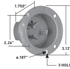
30A Flanged Inlet & Outlet
