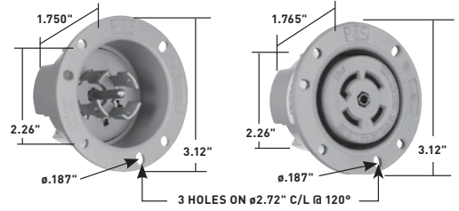
30A Flanged Inlet & Outlet
