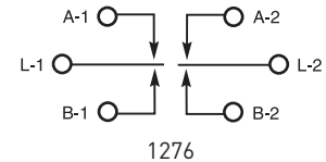
Double Pole Double Throw
