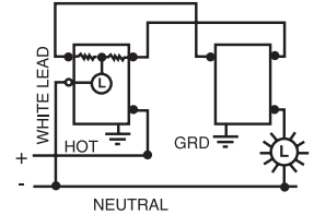
3-Way Lighted Toggle Switch
