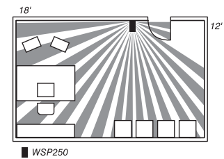
Placement for PIR wall switch sensor
