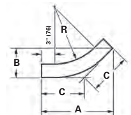
45° Vertical Inside
