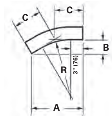
30° Vertical Outside
