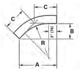
45° Vertical Outside
