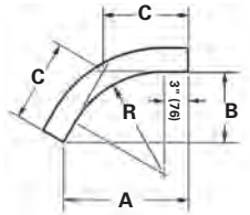
60° Vertical Outside
