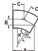
30° Horizontal Bend
