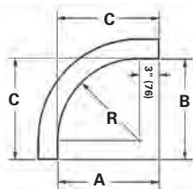
90° Vertical Outside
