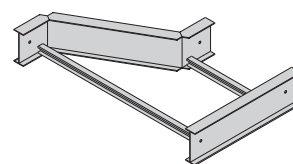
Right Reducer - RR
