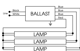
For Two Lamp Operation, Insulate one blue lead to 600V
