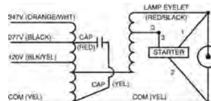
Wiring Diagram 9
