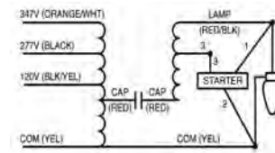
Wiring Diagram 3
