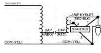
Wiring Diagram 14
