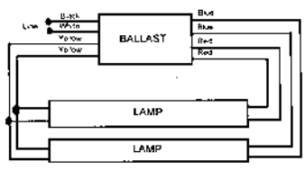
For One Lamp Applications, individually cap blue leads, Insulate to 600V
