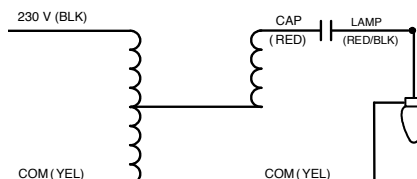
Wiring Diagram 18
