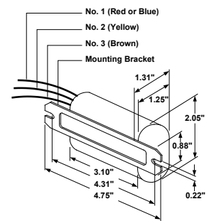
Ref. Drawing 29
