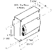
REFERENCE DRAWING 5
