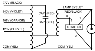
Wiring Diagram 10
