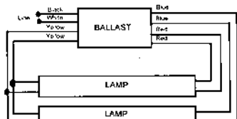
For One lamp Operation, Individually Cap blue leads, Insulate to 600V
