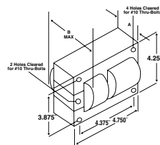
REFERENCE DRAWING PC2
