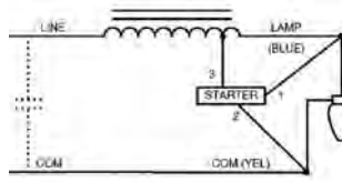
Wiring Diagram 7
