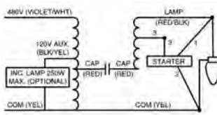
Wiring Diagram 4
