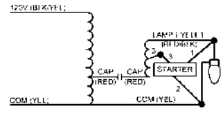
Wiring Diagram 14
