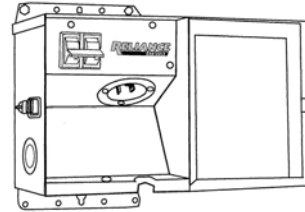
CSR202 & CSR302 - 11 lbs 8.75'h x7.25"w x6.5"d
