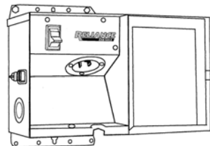
CSR201 & CSR301 - 11 lbs 8.75'h x7.25"w x6.5"d
