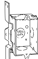
CWV 1/2 CV bracket recessed 7/8"
