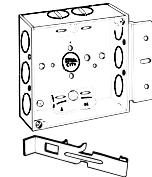
52151 MS N* MS bracket for 1 1/4", 2 1/4", 3 3/4", 4"
