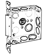
52151-V-1/2 & 3/4 SV Bracket mounted flush
