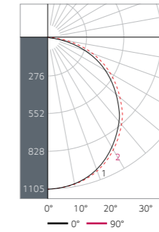
Coefficients of utilization - zonal cavity method
