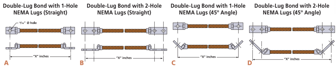
Double-Lug Bond Part No.*
