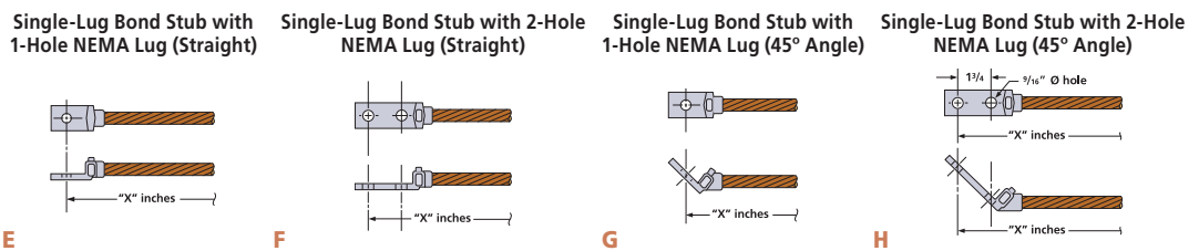
Single-Lug Bond Stub Part No.*
