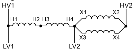
Wiring Diagram 3
