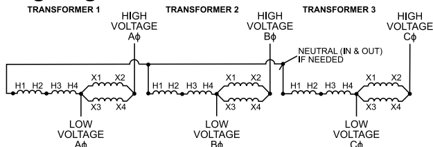
Wiring Diagram 7
