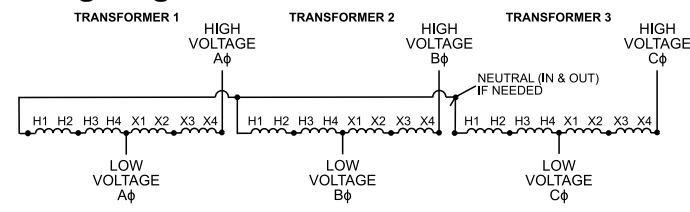
Wiring Diagram 8
