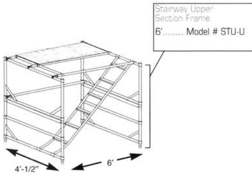
Upper Section
