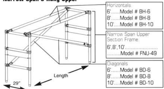
4' High Upper Section Narrow Span 3 Rung Upper
