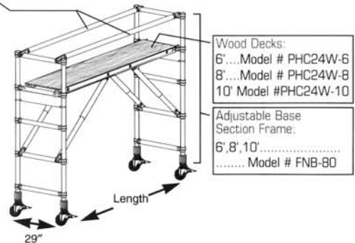
Base Section Narrow Span Hi-Clearance Base
