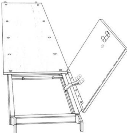
Access Door Platform Board
