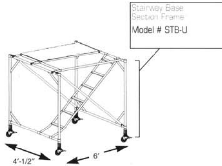
Base Section Adjustable Stairway Scaffold
