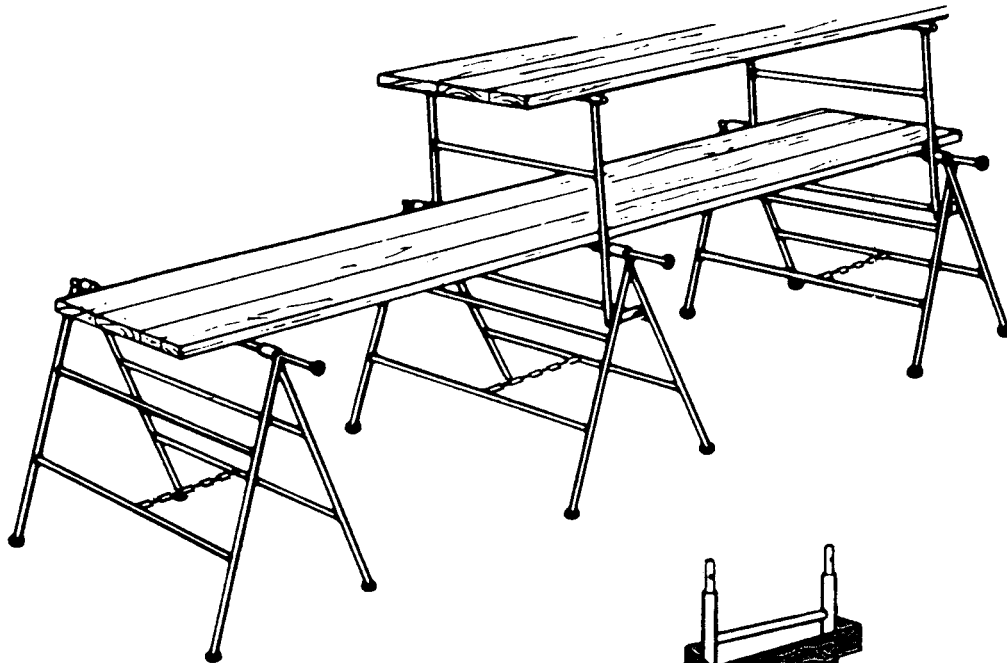
FOLDING TRESTLES 2', 3', 4' & 6' Folding Trestle Extensions 2' & 3'
