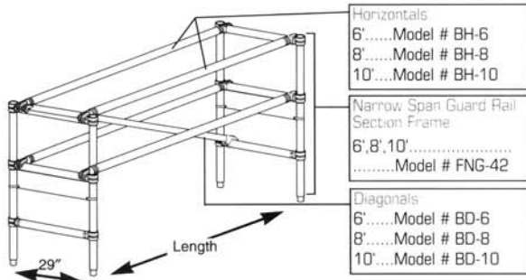
3-1/2' High Guard Rail Narrow Span
