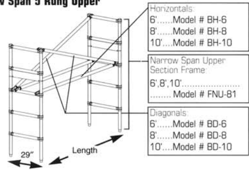
6'9" High Upper Section Narrow Span 5 Rung Upper
