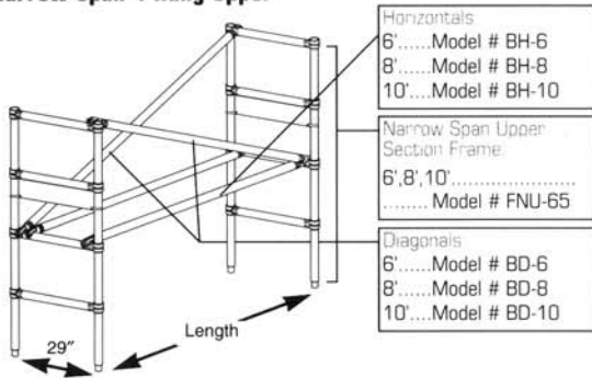
5-1/2' High Upper Section Narrow Span 4 Rung Upper
