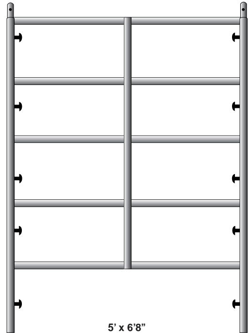
5' x 6'8" DOUBLE LADDER BOX SCL568DB
