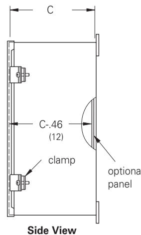
Cover Clamp Layout
