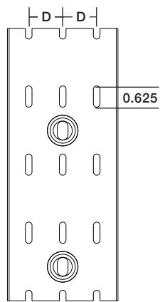
Pattern for 2", 2-1/2", 3", 4" & 6"
