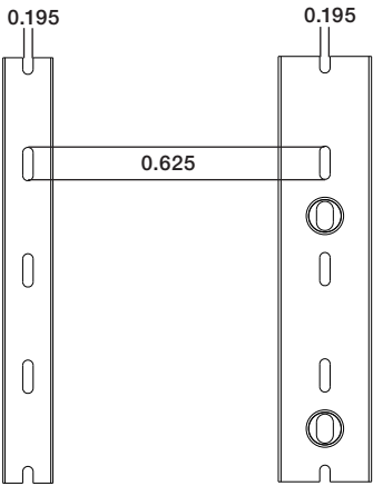
Pattern for 3/4" & 1"
