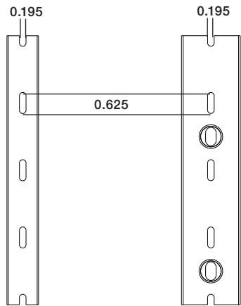
Pattern for 3/4" & 1"
