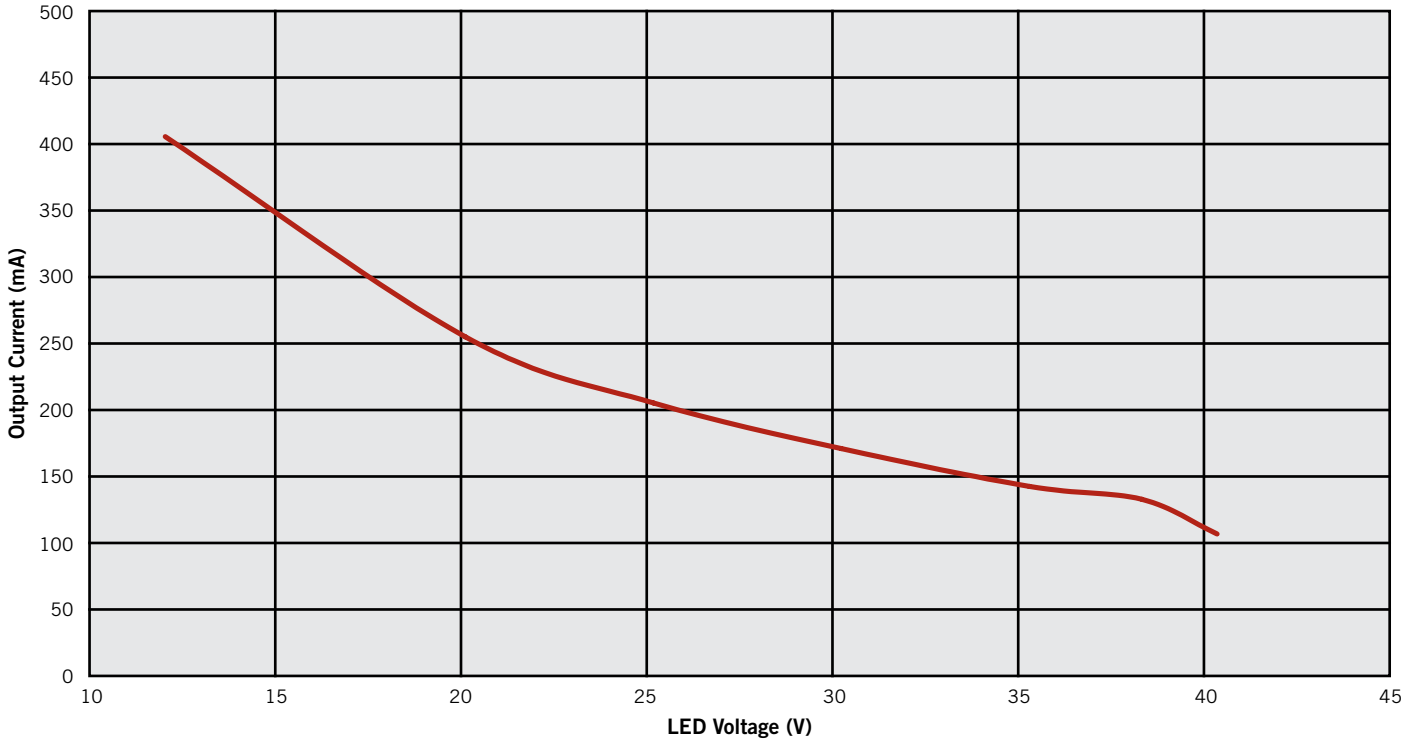
5 WATT OUTPUT CURVE
