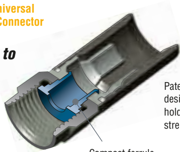
Compact ferrule
