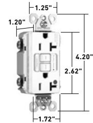
Dimensions for 20 Amp
