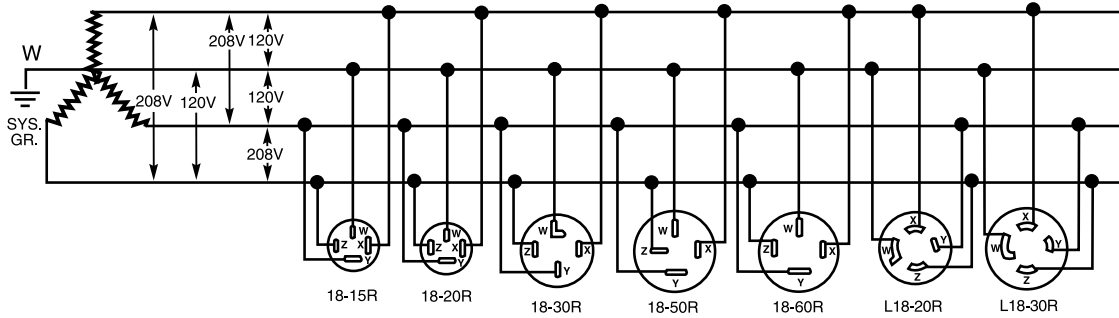
3 \phi Y120V/208V
