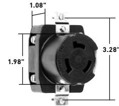
Corrosion-Resistant Receptacle
