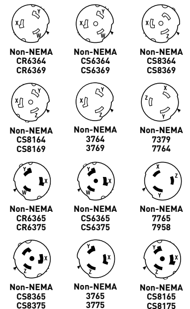
Corrosion-Resistant Flanged Inlet
