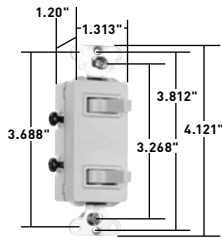
Paddle-Style Combination Switch
