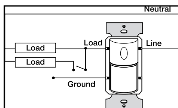
Manual Bi-level Lighting – WS250
