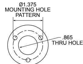
Series 15 Panel Mount Family Cut-out
