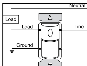
Single Level Lighting – WS250
