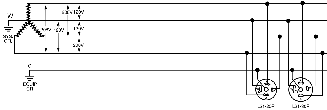
3 \phi Y120V/208V
