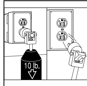
Abrupt Plug Removal Test
