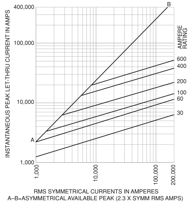
Current Limitation Curves—LPN-RK (250V)
