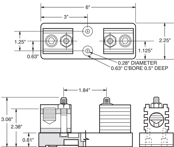
Figure 5. 201A to 400A
