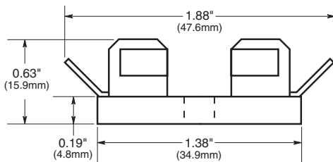
Series 3828 Solder Terminals Fuseblock for 1/4" x 1" Fuses (6.4mm x 25.4mm)
