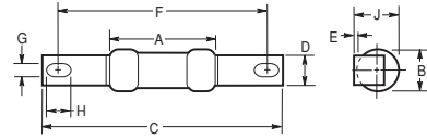
H07C (Offset Blades)
