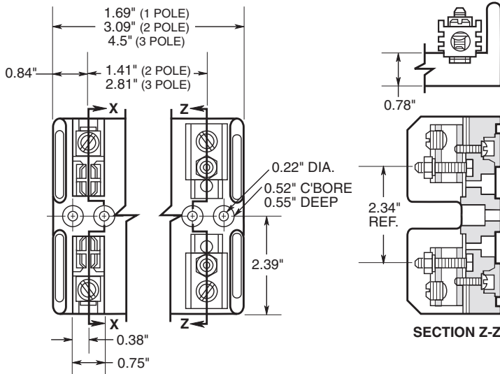
Figure 3. 61A to 100A
