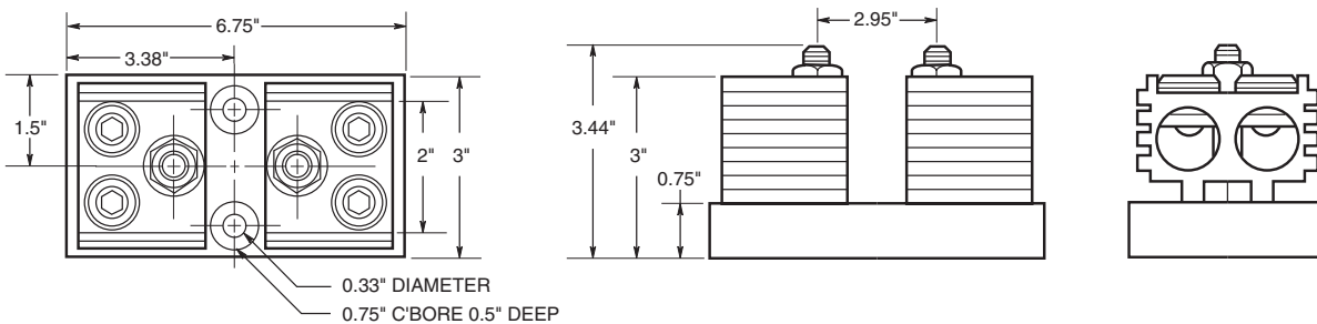
Figure 6. 401A to 600A
