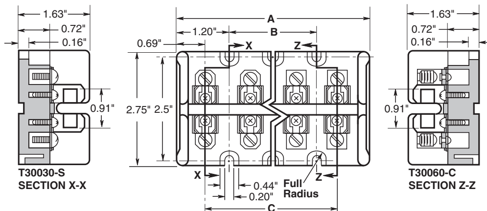
Figure 1. ½A to 60A
