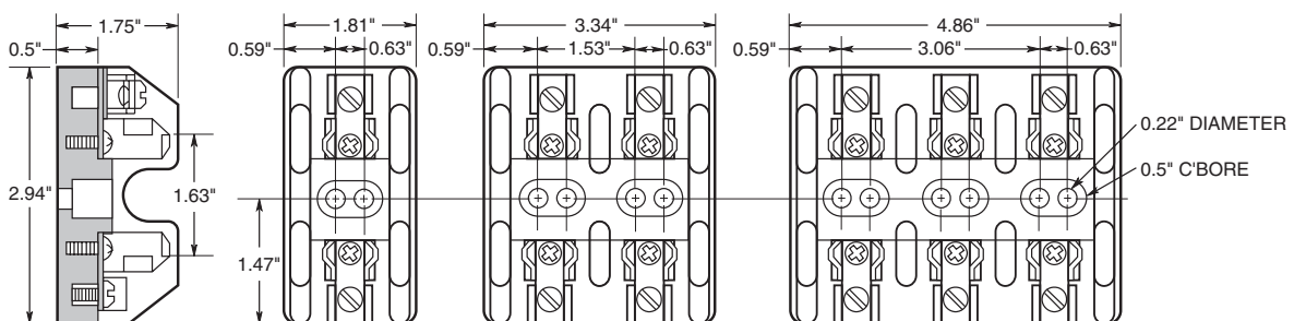
Figure 2. 31A to 60A
