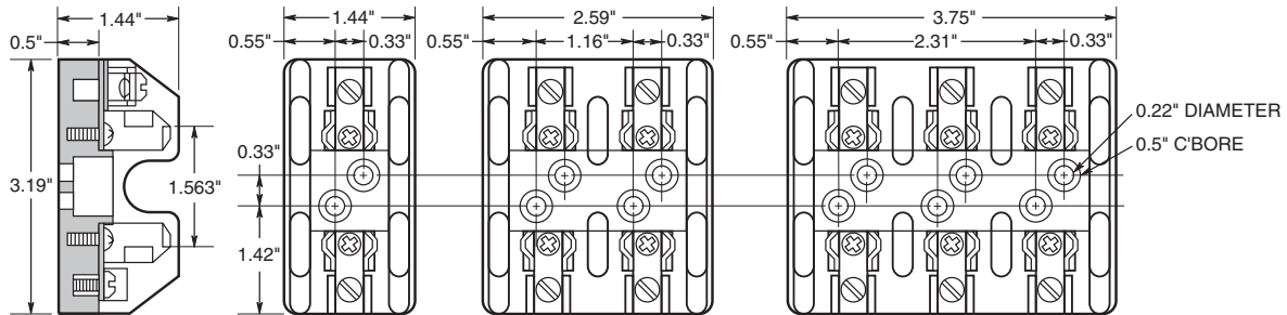
Figure 1. 1/2A to 30A
