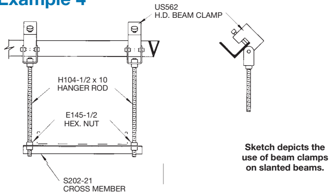
Trapeze with channels as cross members using beam clamps and hanger rods.
