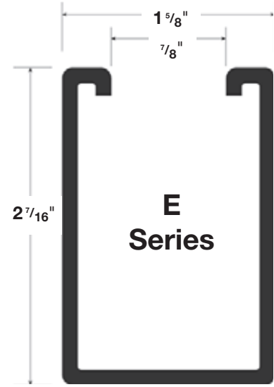
E Series E1200 12 gauge
