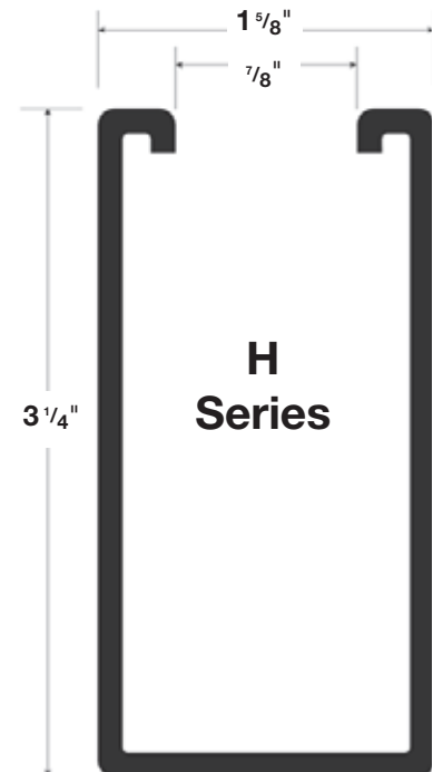
H Series H1200 12 gauge
