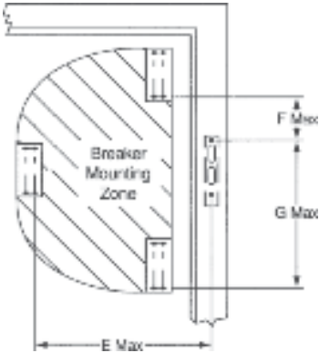
Circuit Breaker Mounting Zone Dimensions
