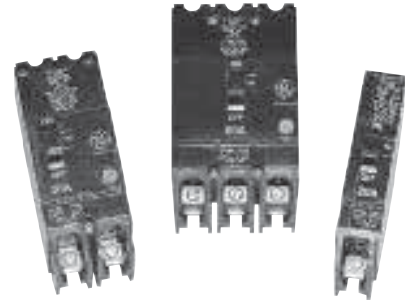
1- 2- and 3-pole TEY/TEYF breakers
