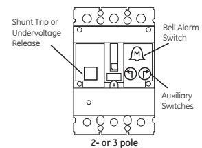
Mounting Locations
