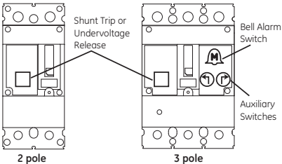
Mounting Locations
