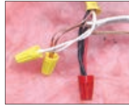
OPEN SPLICE
