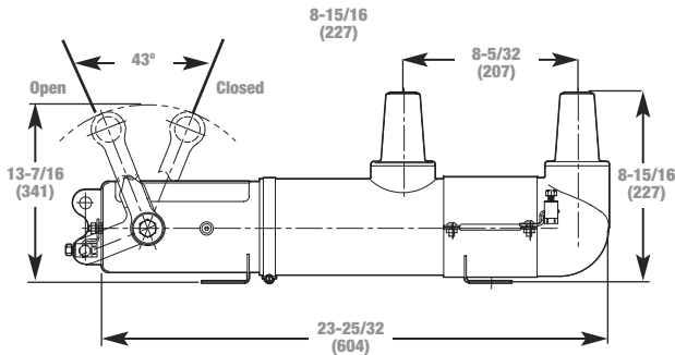
(4) Mounting Holes, 5/8 in. Dia. x 7/8 in. (16 x 22 mm)
