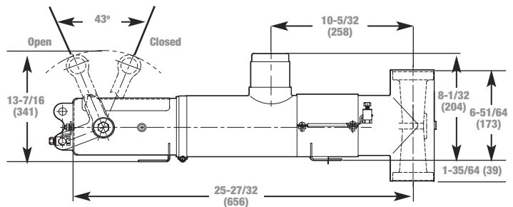
(4) Mounting Holes, 5/8 in. Dia. x 7/8 in. (16 x 22 mm)
