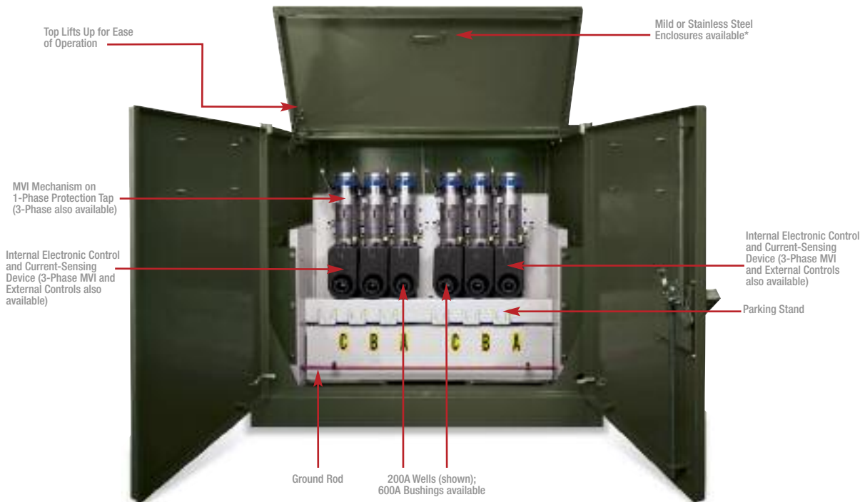
Padmount Unit: Tap (Load) Side
