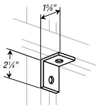
CAT. NO. AB201
