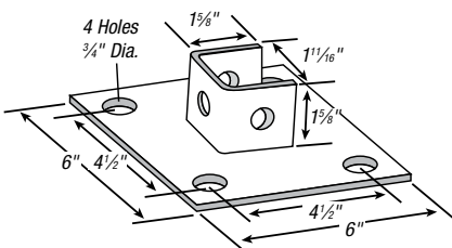
CAT. NO. AP-231SQ
