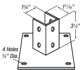
CAT. NO. AP-232
