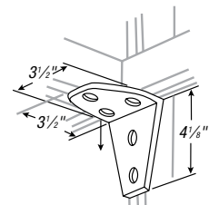
CAT. NO. AB216
