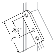
CAT. NO. AB240
