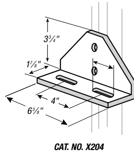
CAT. NO. X204 Slot size is 9/16" x 1 1/2"
