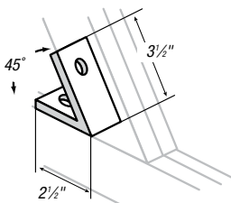
CAT. NO. AB225
