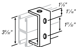
CAT. NO. AB245
