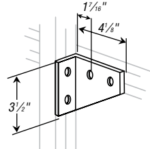
CAT. NO. AB254 L
