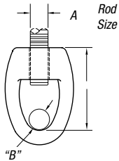
M-117 MI Socket only for S Split Ring Hanger Sizes 3/8" through 7/8" Rod Federal Type 16 SP69 Type 16
