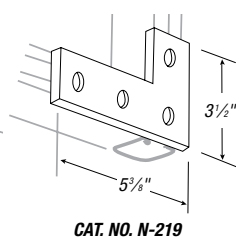
CAT. NO. N-219
