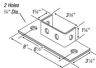
CAT. NO. AP-234FL
