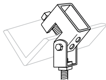
U562 Beam Clamp with Swing Hanger ½" screw included. Rod size: ½" Design load 800 lbs.
