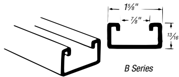
12 gauge B-1200_SS B-1200_T316SS 14 gauge B-1400_SS B-1400_T316SS
