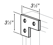
CAT. NO. AB219
