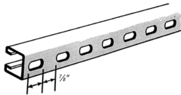
A-1200-HS_AL Slots 2" on center. Slot size 3/16" x 1 1/8"
