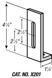
CAT. NO. X201
