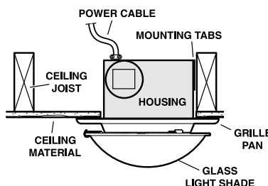
HOUSING MOUNTED DIRECTLY TO JOIST 2x6 (or larger)
