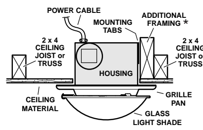
HOUSING MOUNTED TO 2x4 TRUSS
