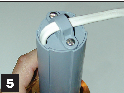
Figure 5 - Secure wire clamp on bottom of tube.
