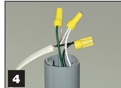
Figure 4 - Connect receptacle wires to NM Cable. Be sure to match wire color(s).
