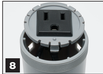
Figure 8 - Remove receptacle by pressing three tabs located on side of tube.
