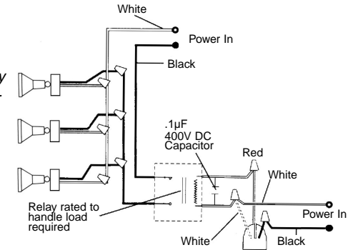
To switch more than rated load (Relay model only)
