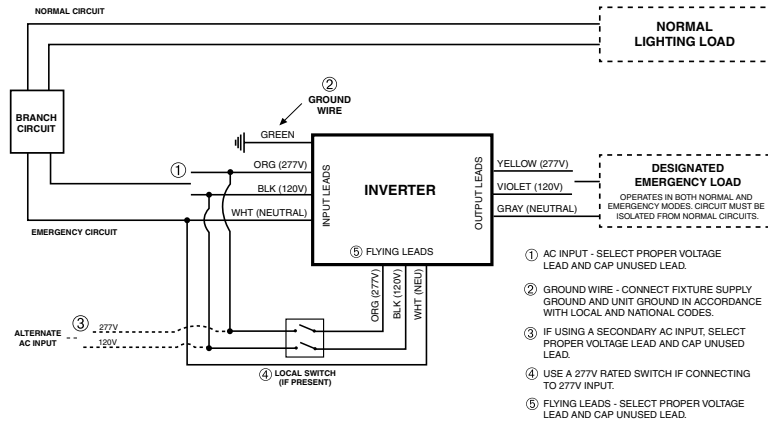
FIGURE 1 - IIS-125 WIRING CONNECTIONS
