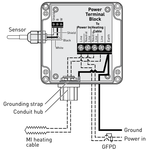
MI heating cable using direct connection
