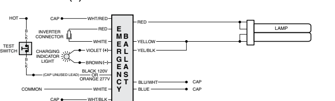
FIG O ONE (1) 36 W - 55 W LAMP WITHOUT AC BALLAST
