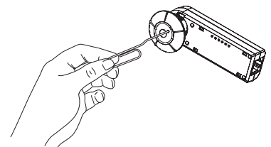
Fig. 9: CONFIG Button
