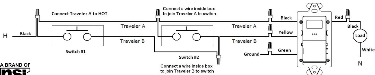
Figure 2 Use momentary switches at all additional locations. Tork #LCS115M
