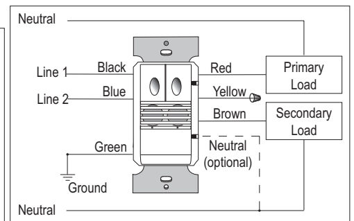
DSW-302 and DSW-302-347 Dual Circuit Wiring
