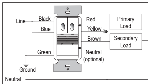
DSW-302 and DSW-302-347 Bi-Level Wiring
