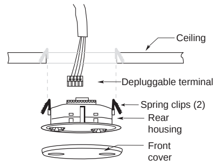
Ceiling Mount
