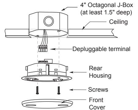
J-Box Mount
