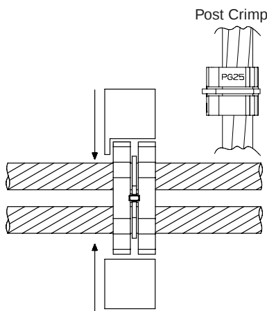
Crimp (1)*
