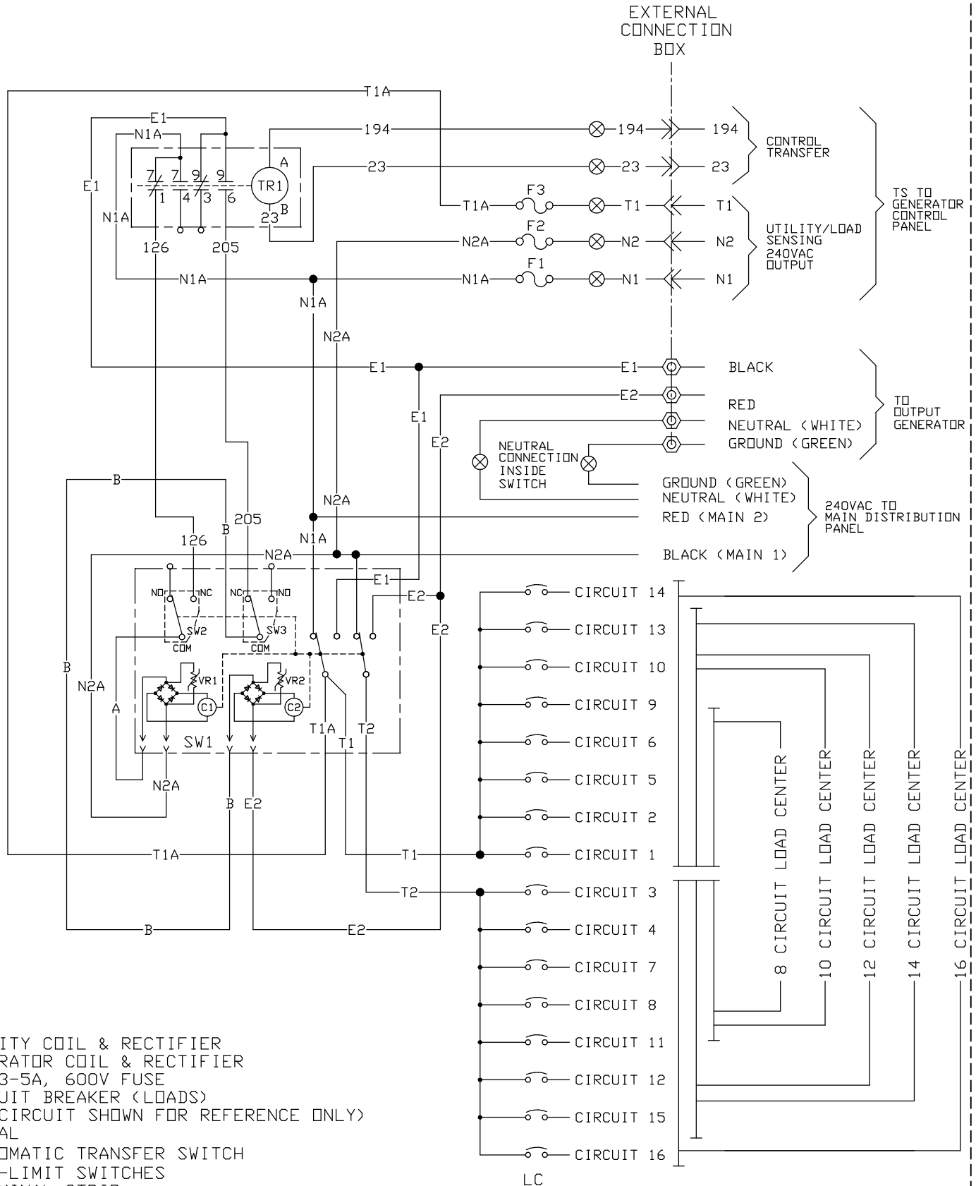
SCHEMATIC - DIAGRAM HSB TRANSFER SWITCH DRAWING #: 0H6386
