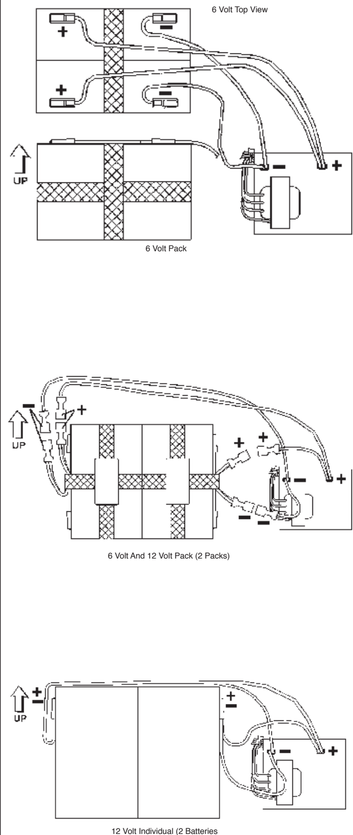
Fig. 6 Double Harness Lead Connection Nickel-Cadmium Batteries
