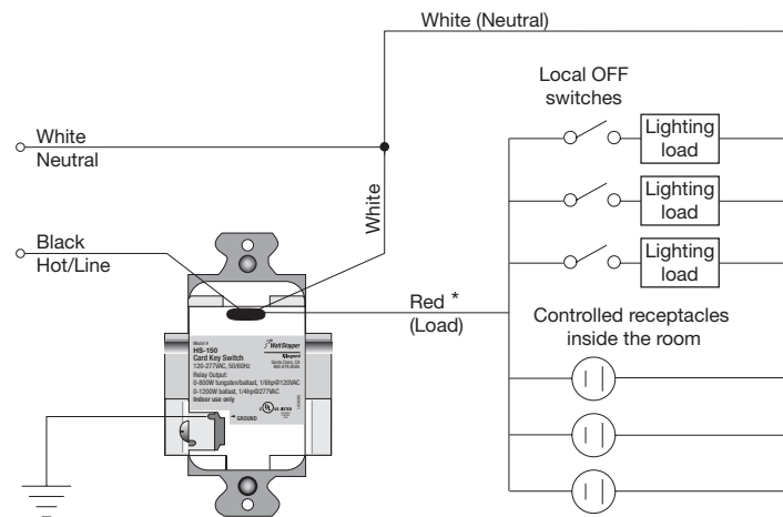
Figure 2: Line voltage wiring
