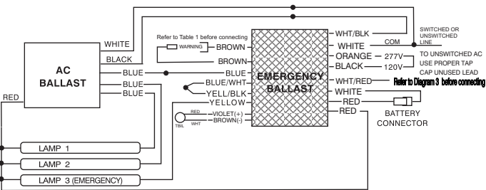
C. THREE (3) LAMP INSTANT START BALLAST
