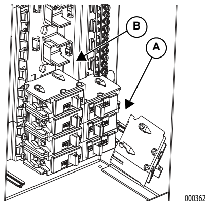
Figure 3-1. Installing Breakers
