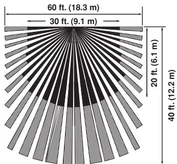
Figure 1 - Field-of-View (Horizontal)
