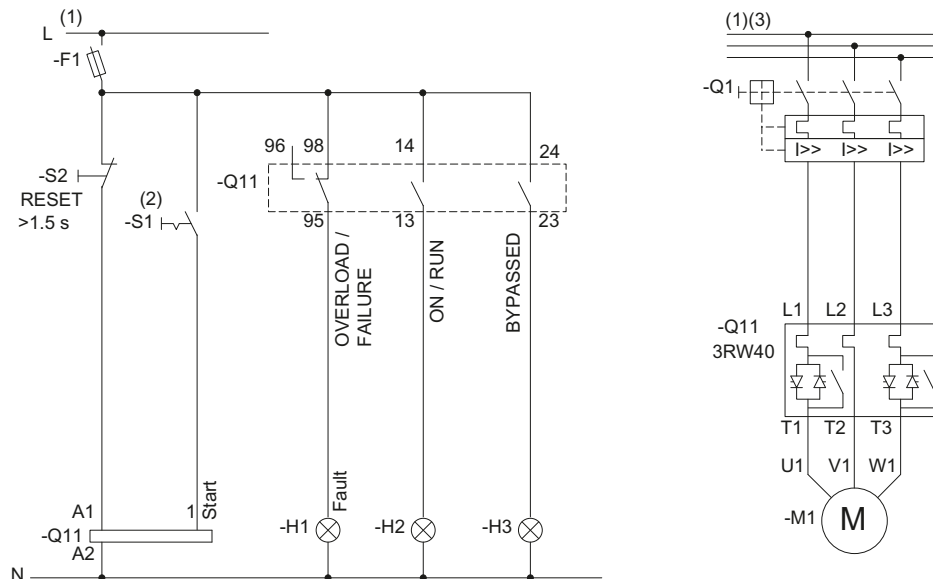
Figure 15-6 Wiring of the 3RW40 2 to 3RW40 4 control circuit and the 3RW40 2 to 3RW40 7 main circuit
