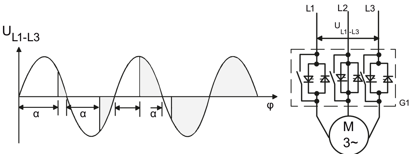
Figure 3-5 Phase angle control and schematic diagram of a two-phase controlled soft starter with integral bypass contacts
