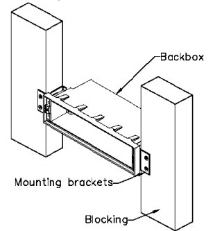
Figure 2 (stud wall)
