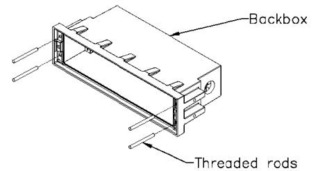
Figure 3 (poured concrete)
