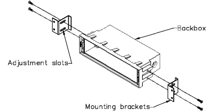
Figure 1 (stud wall)
