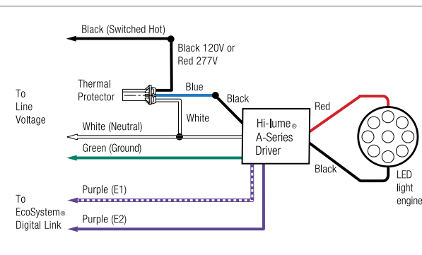
Wiring Diagram for EcoSystem® Digital Control
