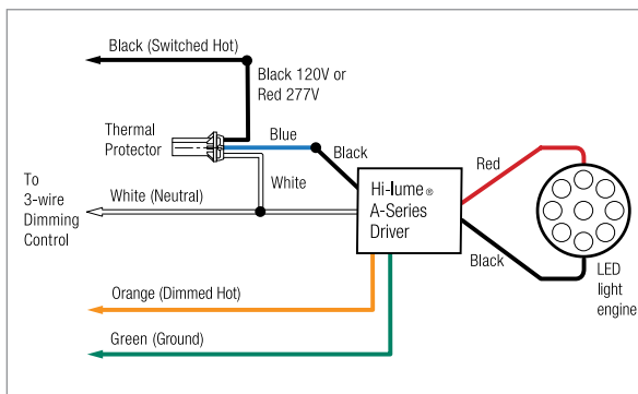
Wiring Diagram for 3-Wire Control
