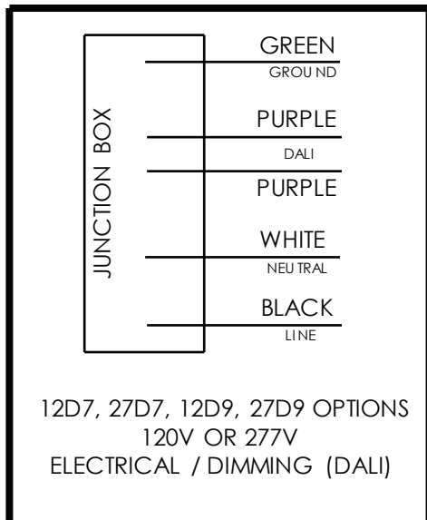
WIRING DIAGRAM-4
