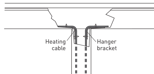
Figure 11. Hanger brackets
