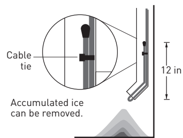
Figure 10. Heating cable in downspout
