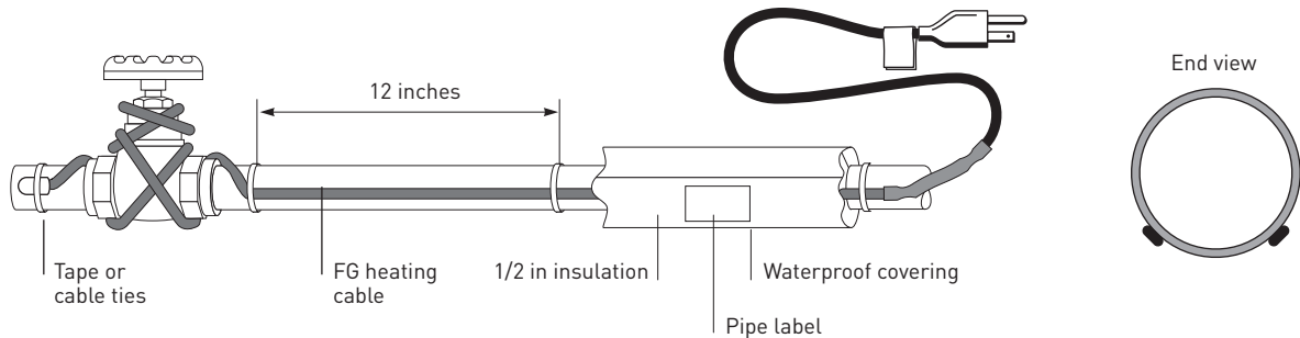
Figure 1. Straight-traced installation
