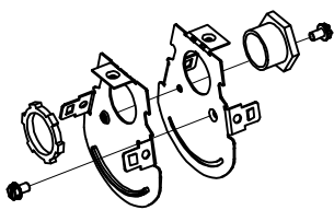
FIG 7: JOINER ASSY
