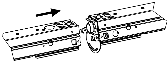
FIG 8: ROW MOUNT CONNECTION
