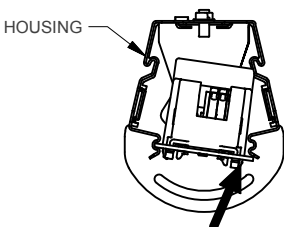
FIGURE 3: BOARD SNAP IN
