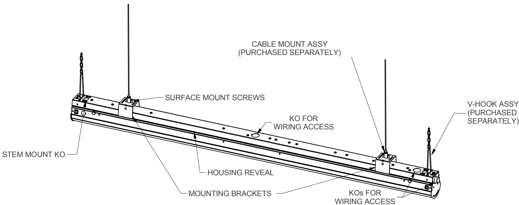
FIGURE 1: STAND ALONE CONFIGURATION
