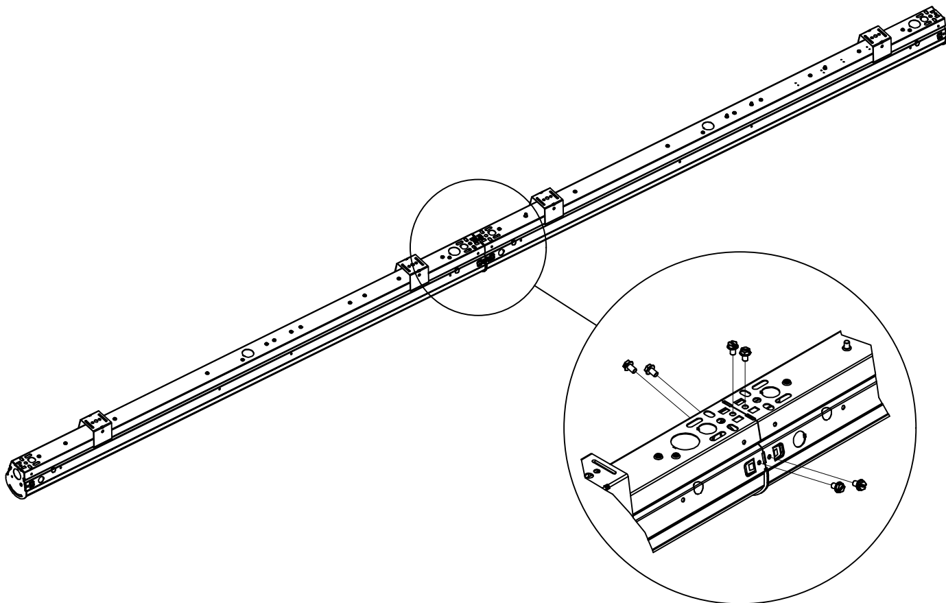
Figure 8: Configuration Mont Row
