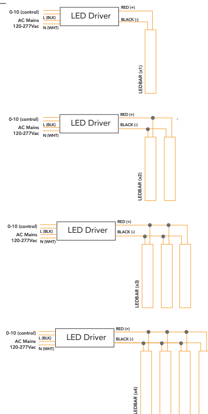
WIRING DIAGRAM
