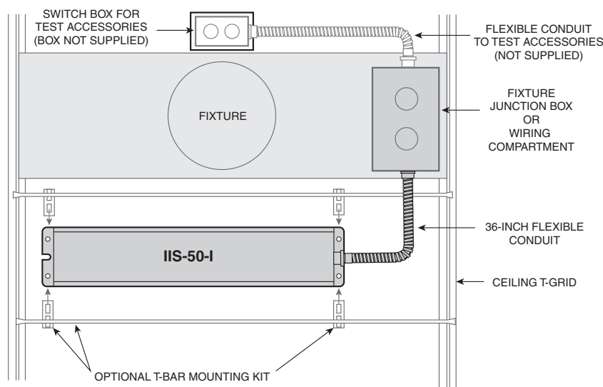
Illustration 1: IIS-50-I and Test Accessory Mounting (Top View)
