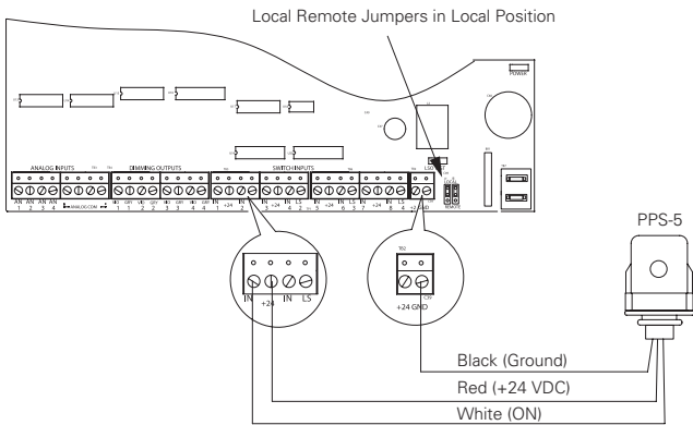
Figure 6. ControlKeeper 4A Connection
