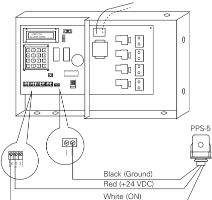
Figure 3. LiteKeeper 4 Connection
