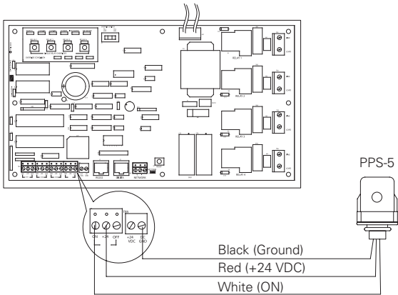
Figure 5. ControlKeeper 4 Connection
