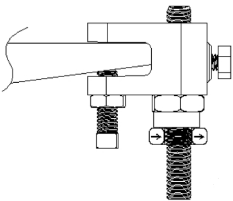
Application With CADDY ROD LOCK Beam Clamp
