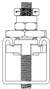
Application With CADDY ROD LOCK Channel Nut
